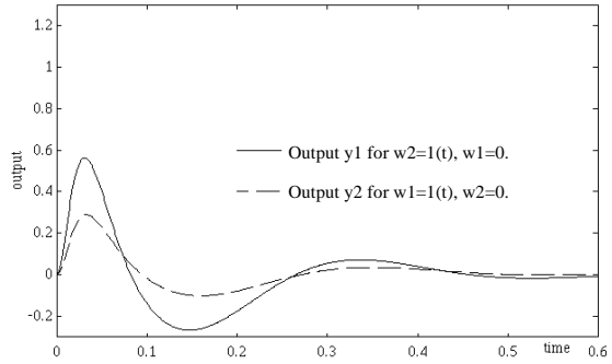
Fig.4 Time responses as a result of coupling.
