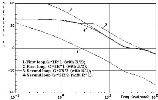
Fig.5 Bode plots of particular loops.
