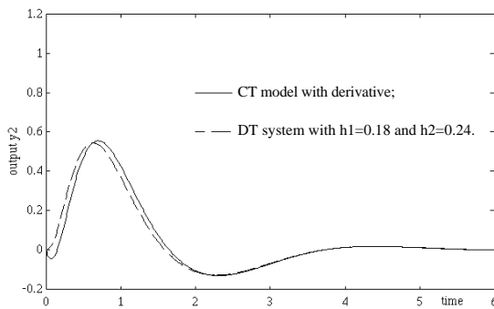
Fig.9 Time responses of y2 for w1=1(t).
