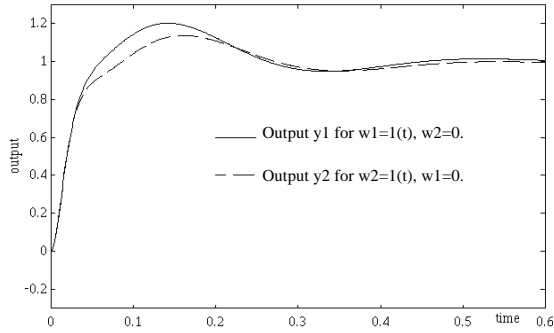
Fig.3 Time responses of the CL systems.
