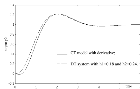
Fig.8 Step responses of the second output.
