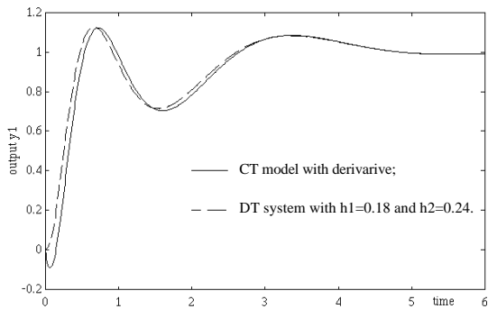
Fig.7 Step responses of the first loop.
