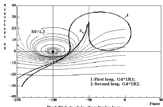
Fig.6 Nichols plots of particular loops.
