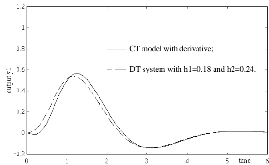
Fig.10 Time responses of y1 for w2=1(t).
