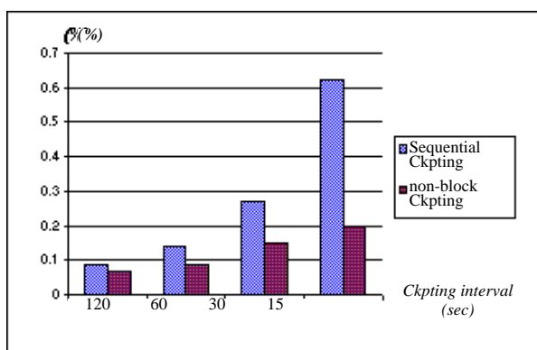
Figure 4.2 Checkpointing overhead
