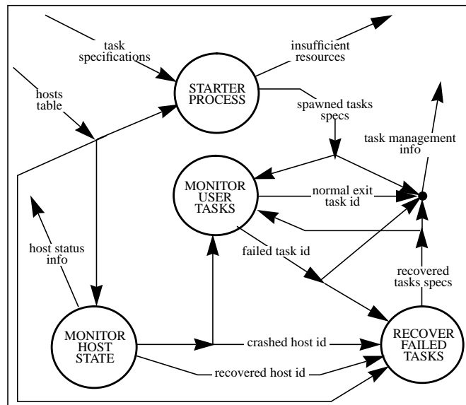
Figure 2.1 The Fault-Tolerant Environment
