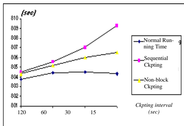
Figure 4.1 Execution Time
