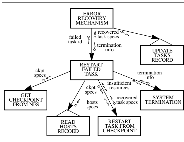
Figure 2.3 The User-Processes Recovery Task
