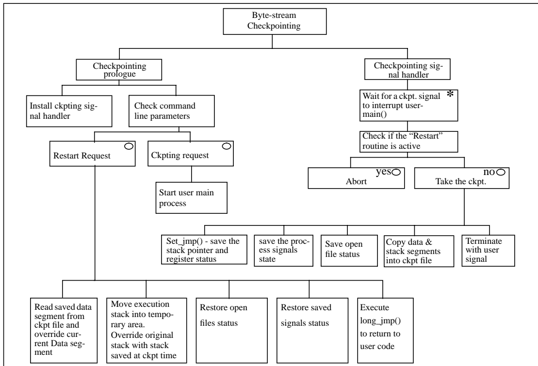
Figure 3.1 The Checkpointing Protocol
