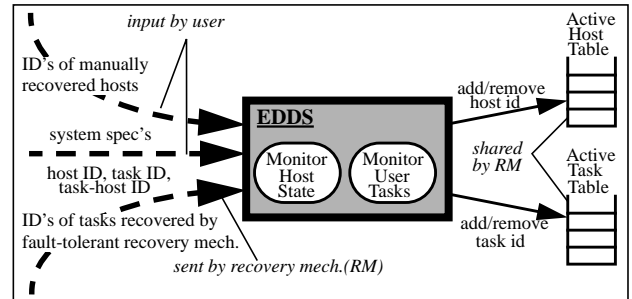
Fig. 2.2 The Error Detection Mechanism
