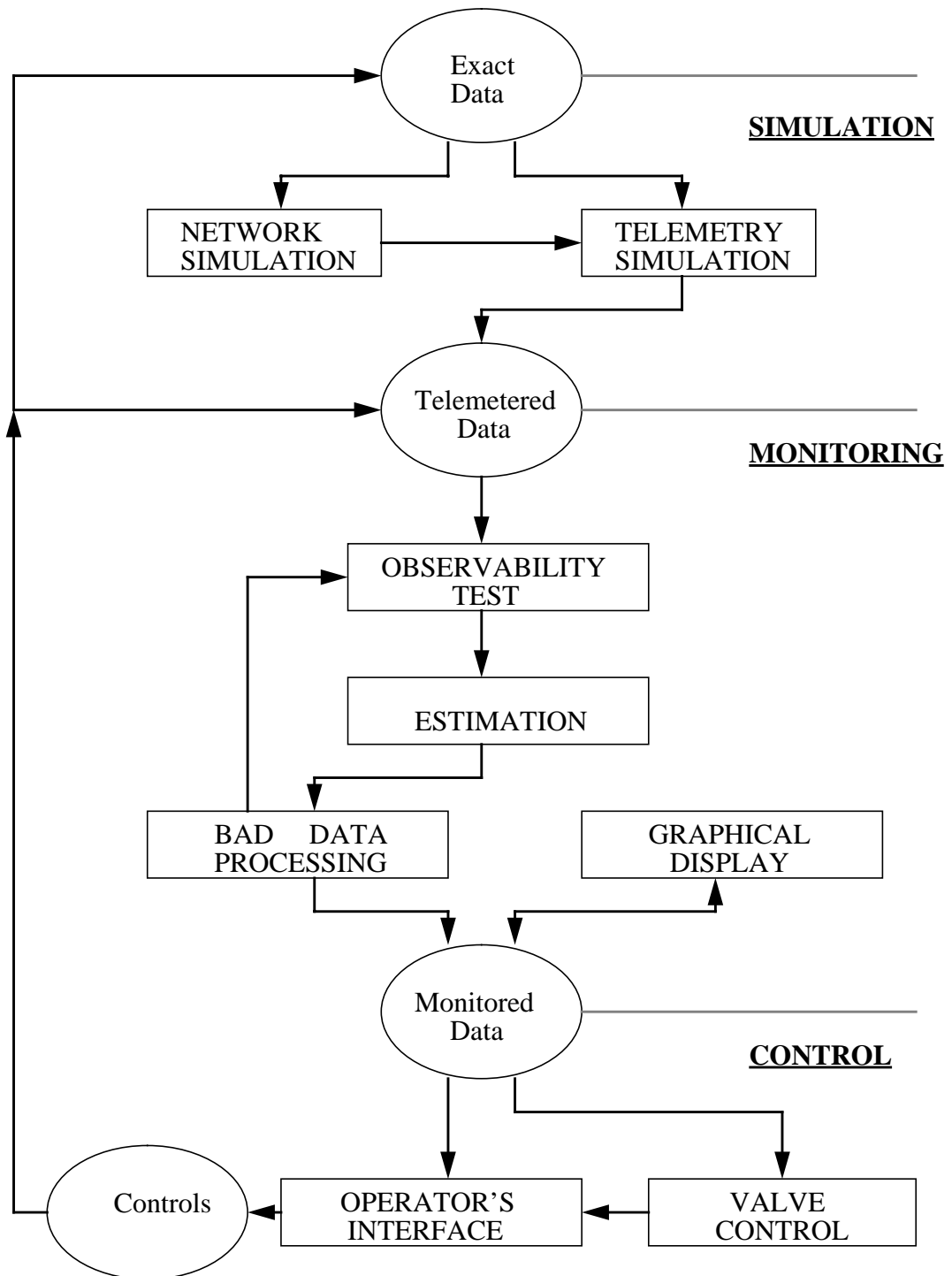
Figure 4. Water network monitoring suite
