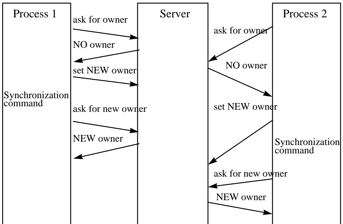
Figure 3. Possible sequence of events leading to lock violation
