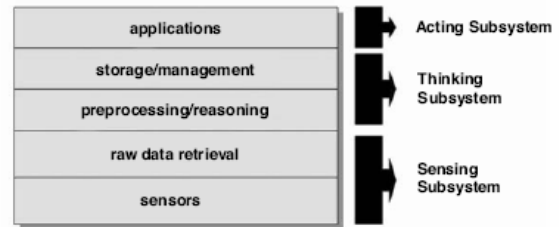
Figure 1. Abstract layered architecture for context aware systems.
