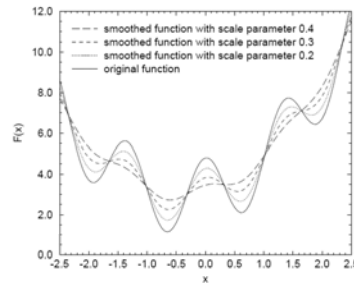
D. Yang, S.J. Flockton, Evolution Algorithms with Coarse-to-Fine Function Smoothing
